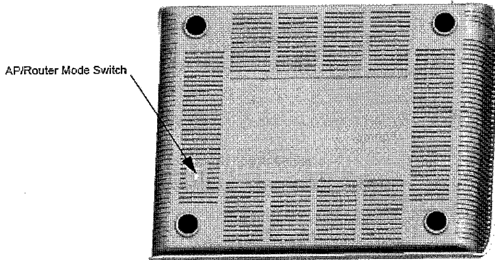
Figure 1-3. Bottom Panel
