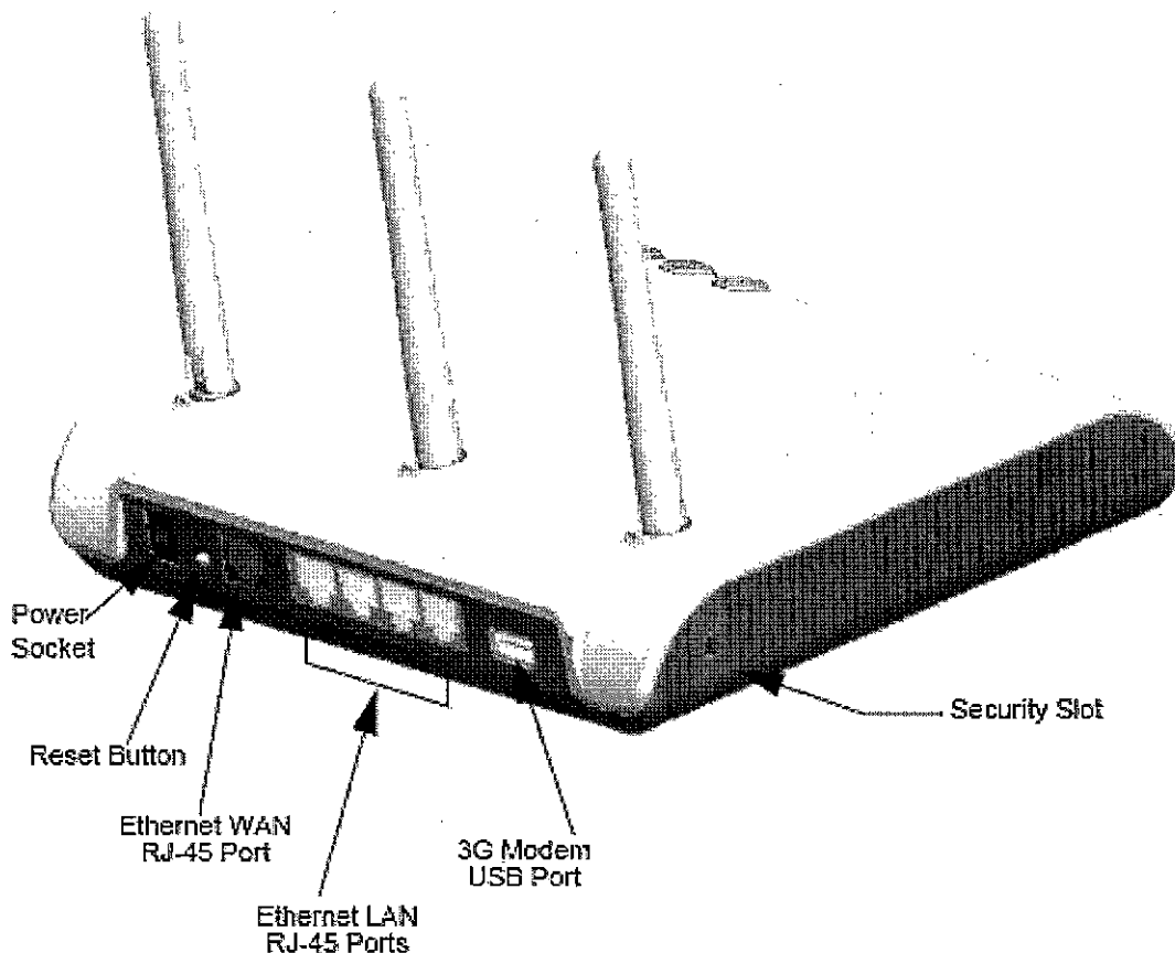
Figure 1-1. Rear Panel
